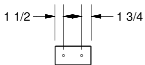
(1) M34 - WALL RAIL - W4L04611 5/8"x3 3/8"x6 3/8" (16x86x162)
