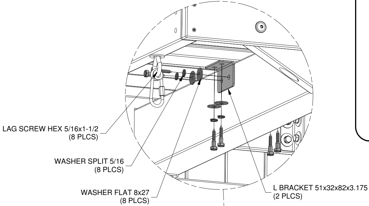
LAG SCREW HEX (8) 5/16x1-1/2 H100066
