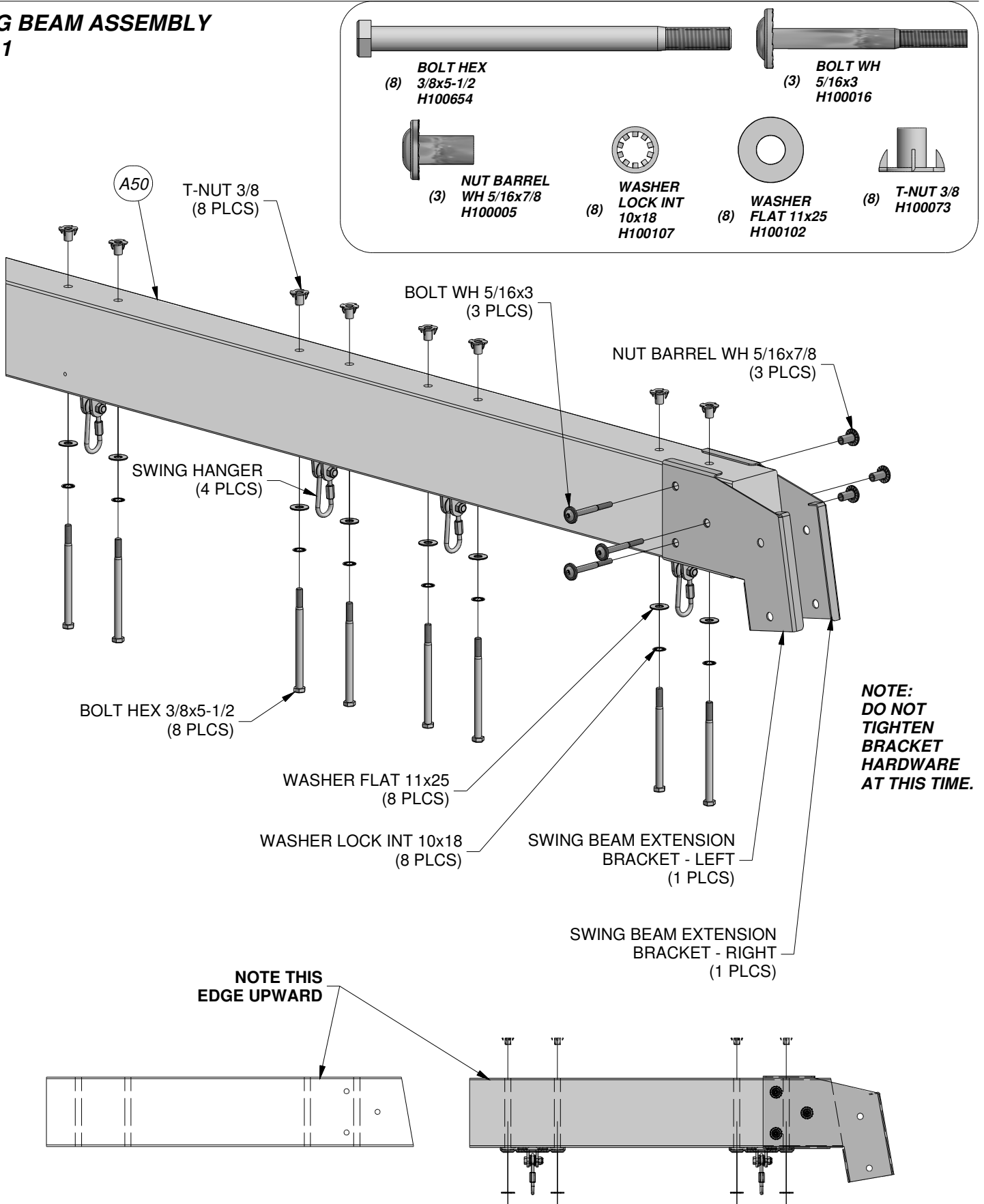
(1) - SWING BEAM EXTENSION BRACKET-LEFT - A100325
